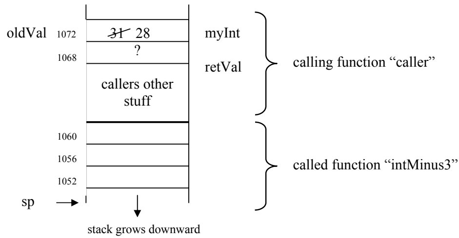
Fig 17.11: call stack layout after oldVal = oldVal - 3 ;
