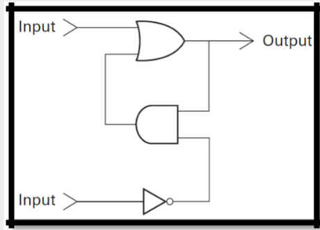
Figure 17: Flip flop
