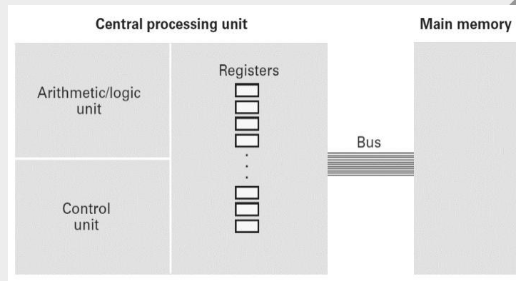
Figure 41: CPU and main memory connected via a bus
