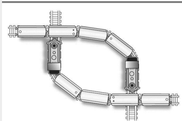
Figure 58: Deadlock Situation
