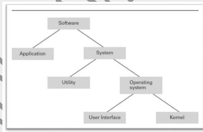
Figure 53: Software Classification
