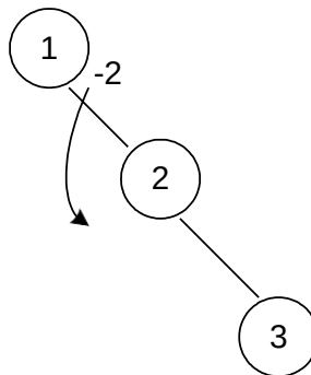
Fig 21.1: insert(3) single left rotation
