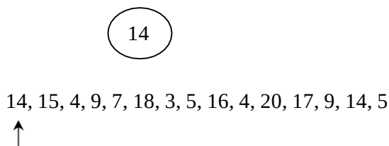
Fig 12.2: First number in the list became the root
