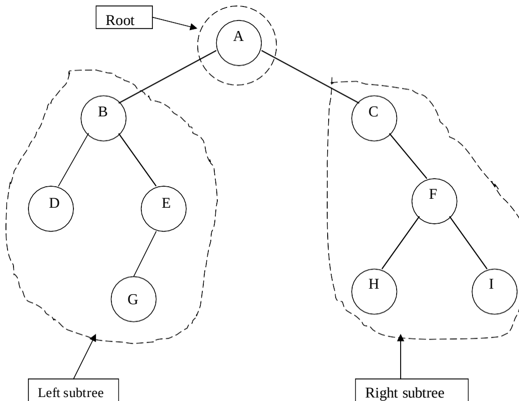
Fig 11.3: Analysis of a binary tree
