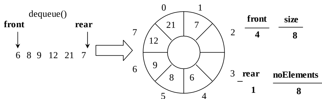
Fig 15. Element removed from the circular array
