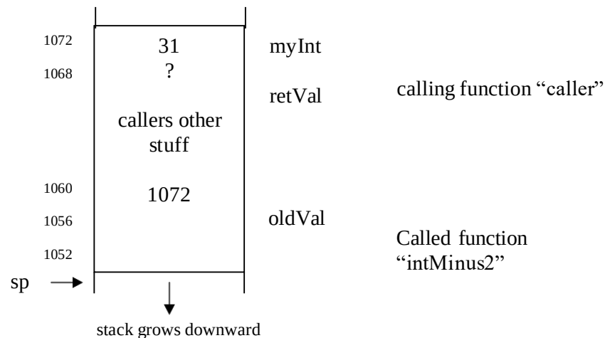
Fig 17.6 call stack layout when intMinus2 is called
