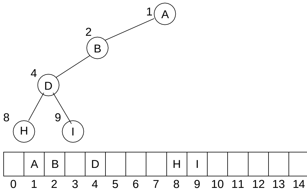
Figure 29.2: Not a complete binary tree
