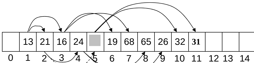
Figure 29.9: inserting new value in a heap
