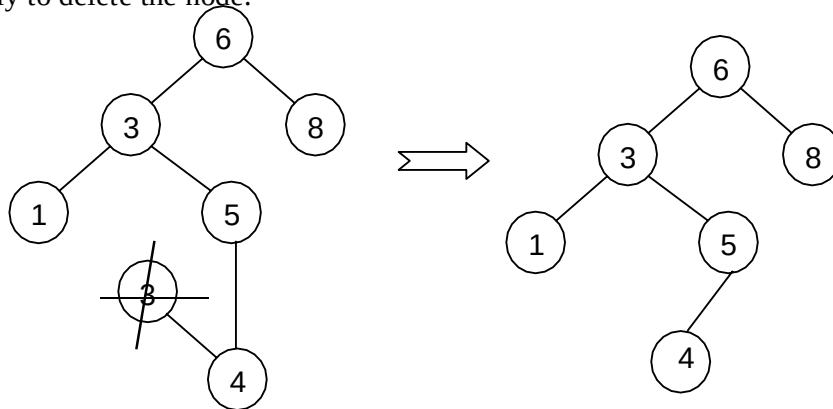
Fig 15.14: delete (2)
