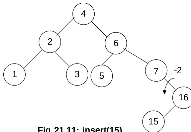
Fig 21.11: insert(15)
