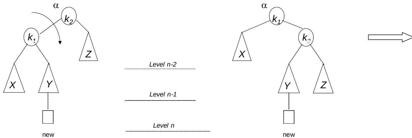
Fig 21.15: Single right rotation fails to fix case 2
