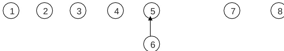
Figure 35.2: After union (5, 6)
