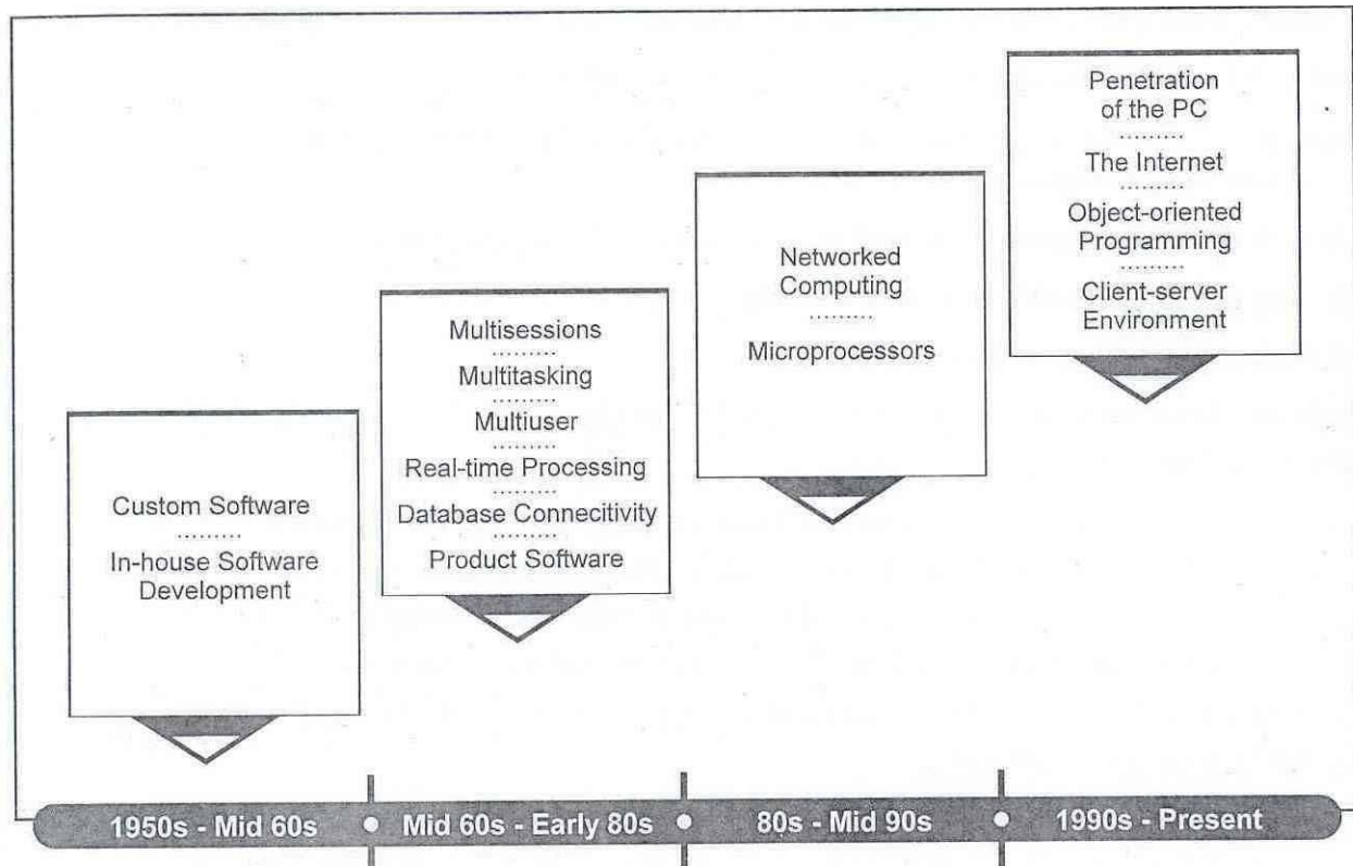
Figure 1.1: Software Evolution
